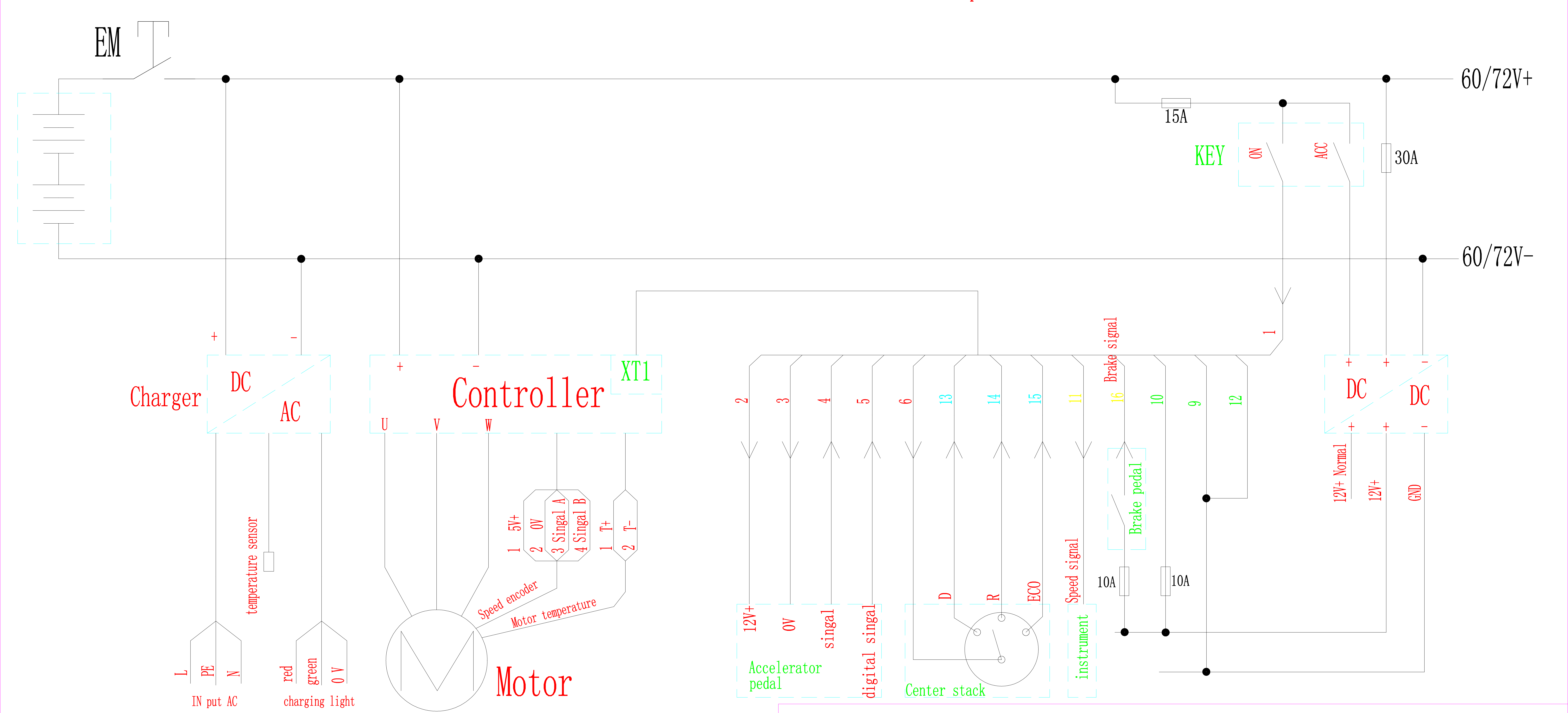
Power system (Lead acid battery) 1
